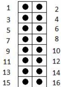
Picture3-1 Interface Picture (HUB75)
